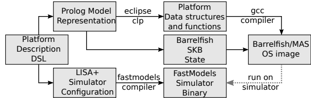
Figure 10: Running Barrelfish/MAS on an ARM FastModels [7] Platform Based on a Hardware Description.
